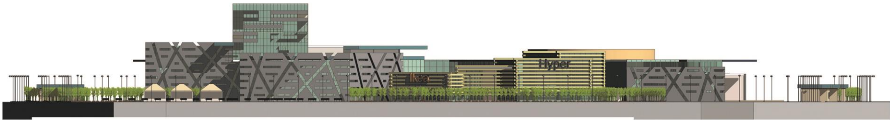
BACK ELEVATION 1:200
