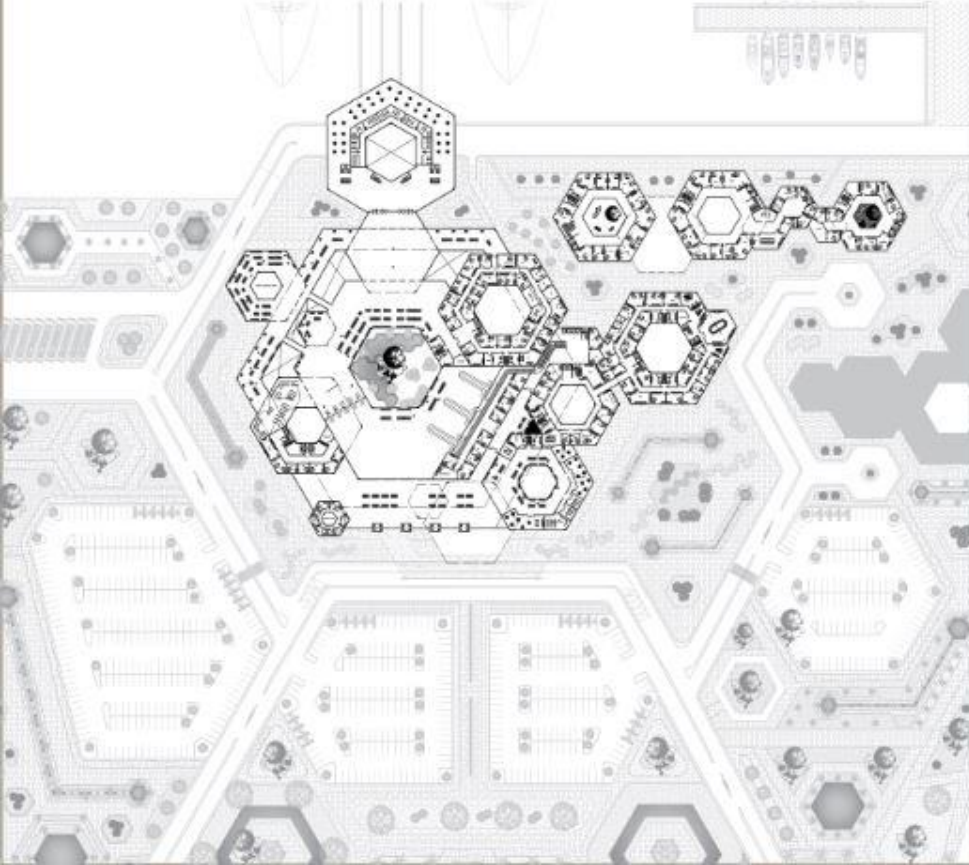
FIRST FLOOR PLAN SCALE 1:500
